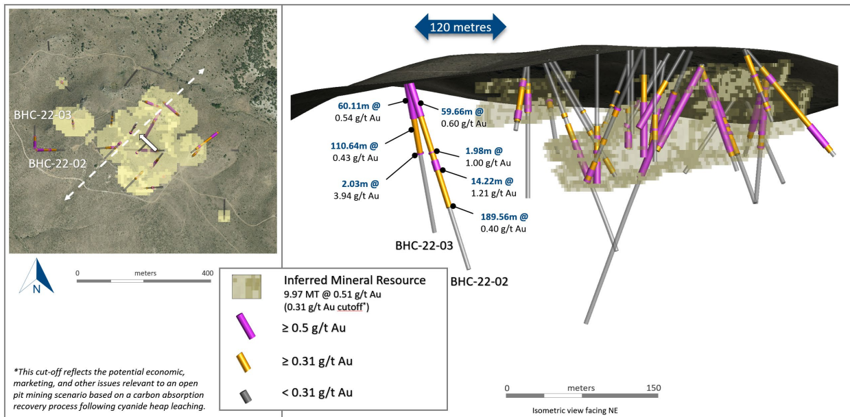
Figure 2: Cross-Section demonstrating assay results for BHC-22-02 and BHC-22-03
